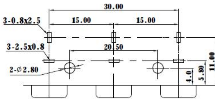
PCB LAYOUT
